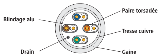
S/FTP
